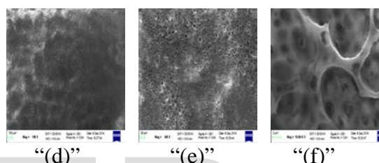
Figure 2: SEM membrane PVA0.5040 g Enzyme-Coating I magnification (a) 100x, (b) 500x, (c) 10000x
