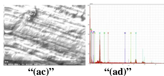
Figure 12: SEM and EDX analysis of PVA 0.0350 g Dyeing enzyme 2x Coating II 1x
