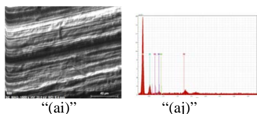
Figure 15: SEM and EDX analysis of PVA 0.0350 g Dyeing enzyme 5x Coating II 1x
