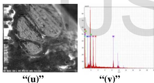
Figure 8: SEM and EDX analysis of PVA 0.5040 g Dyeing enzyme 3x Coating I 1x
