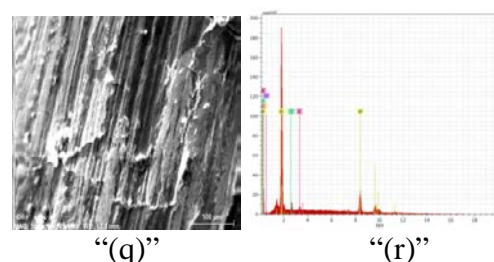
Figure 6: SEM and EDX analysis of PVA 0.5040 g Dyeing enzyme 1x Coating I 1x
